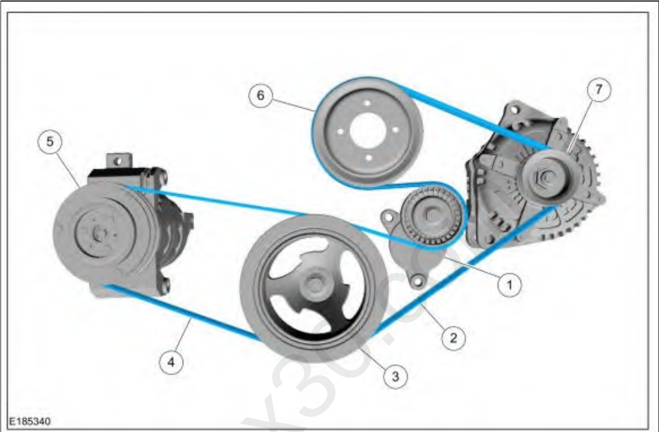
Fig 1: View Of Drive Belt Routing And Pulley
